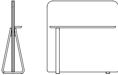
Theo short space divider width 1215 depth 380 height 1240
