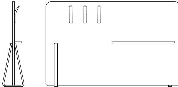
Theo long space divider width 2400 depth 380 height 1525
